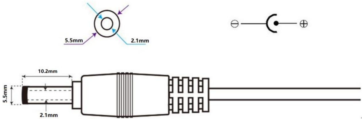
Figure 988: Power Adapter
