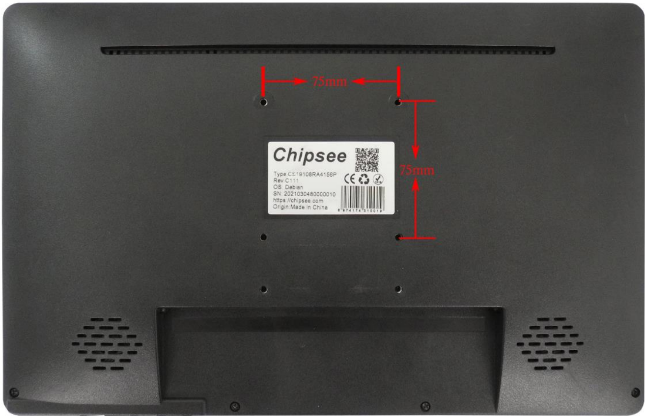
Figure 998: VESA mounting
