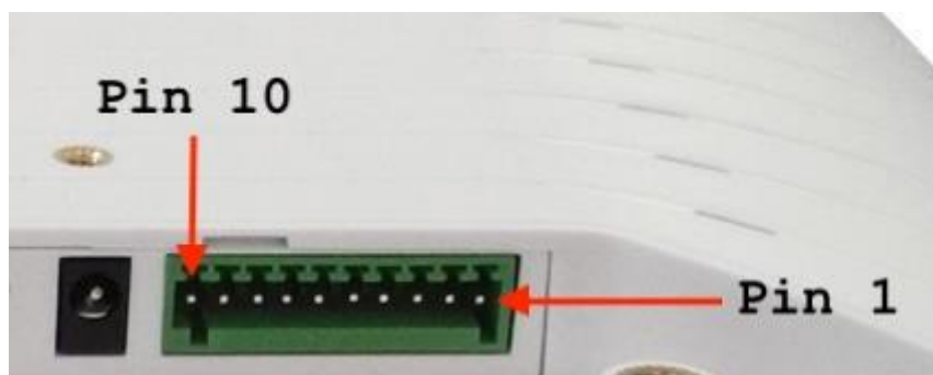
Figure 981: RS232/RS485/Relay Connector
