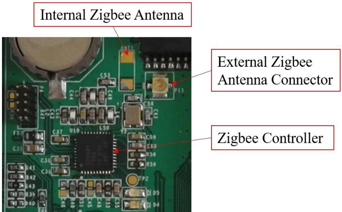
Figure 952: Zigbee controller
