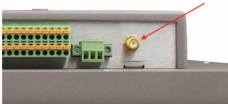
WiFi+BT Antenna
