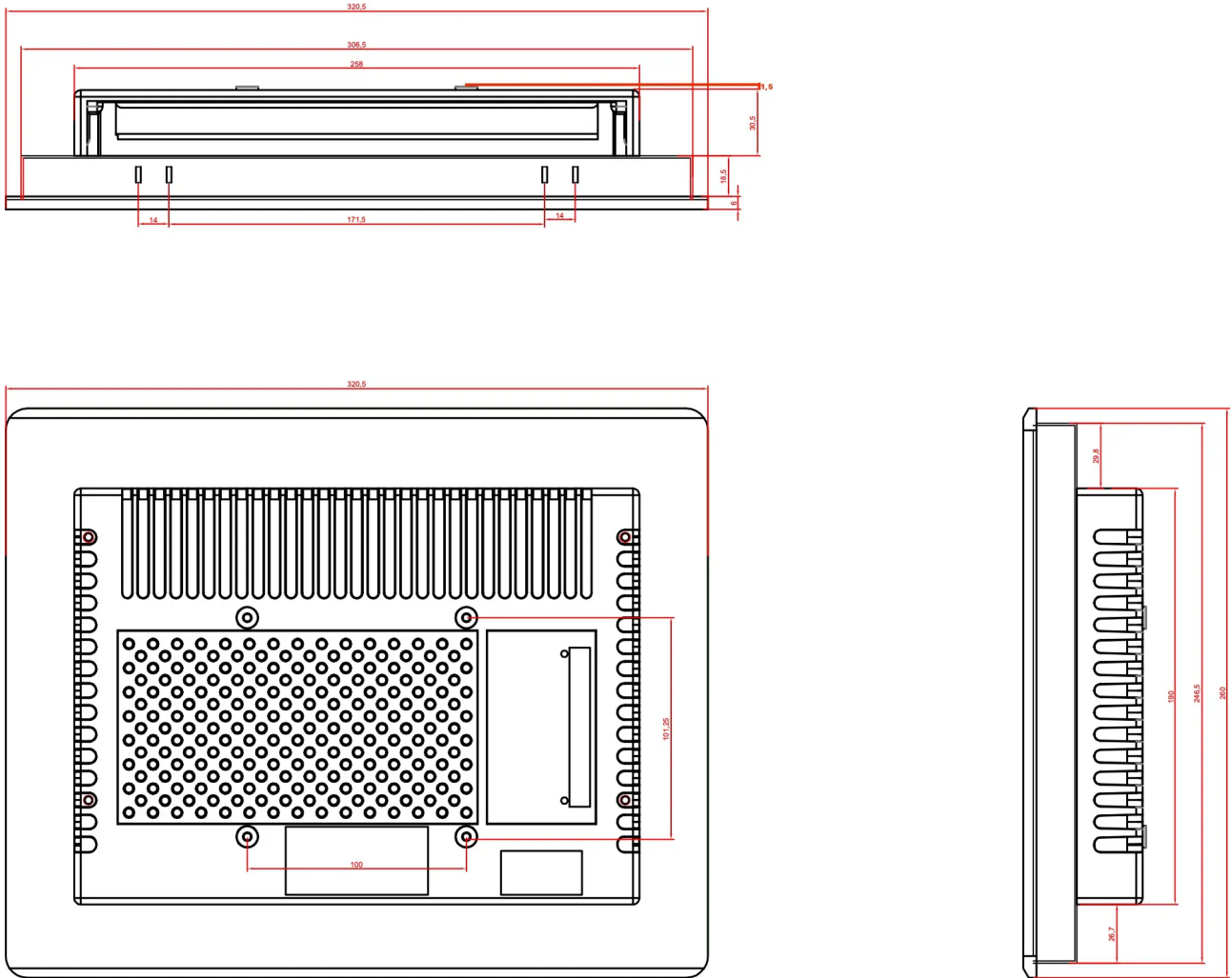
Figure 946: CS10768RA4121P Technical Drawing
