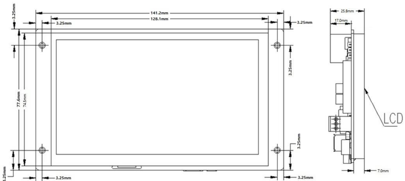
Figure 926: CS12720RA4050E Technical Drawing
