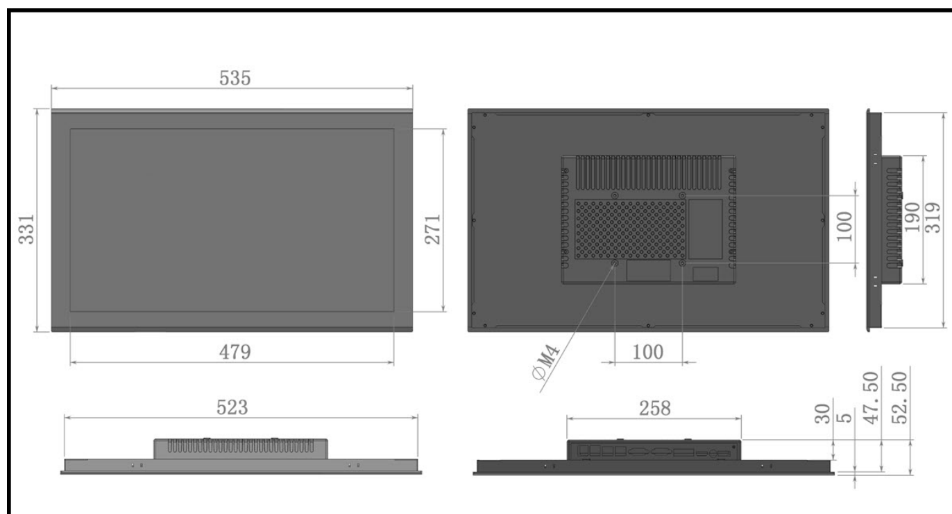
Figure 889: PPC-J1900-215-C Technical Drawing
