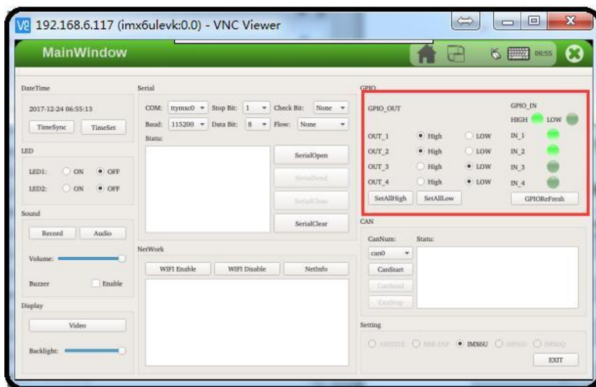
Figure 376: GPIO Test
