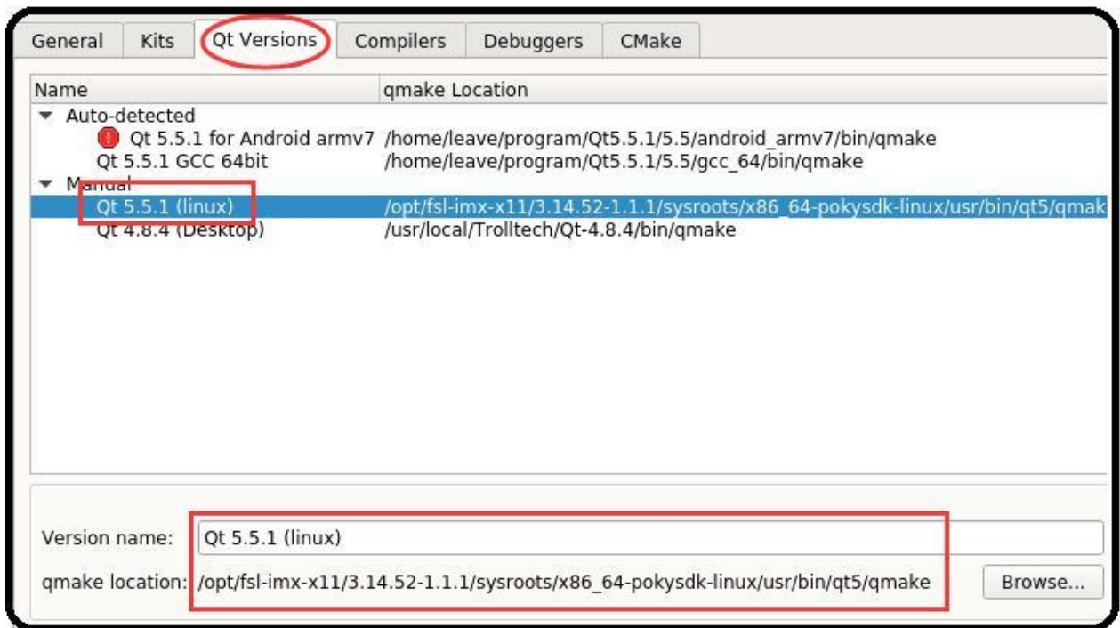
Figure 381: Qt Versions
