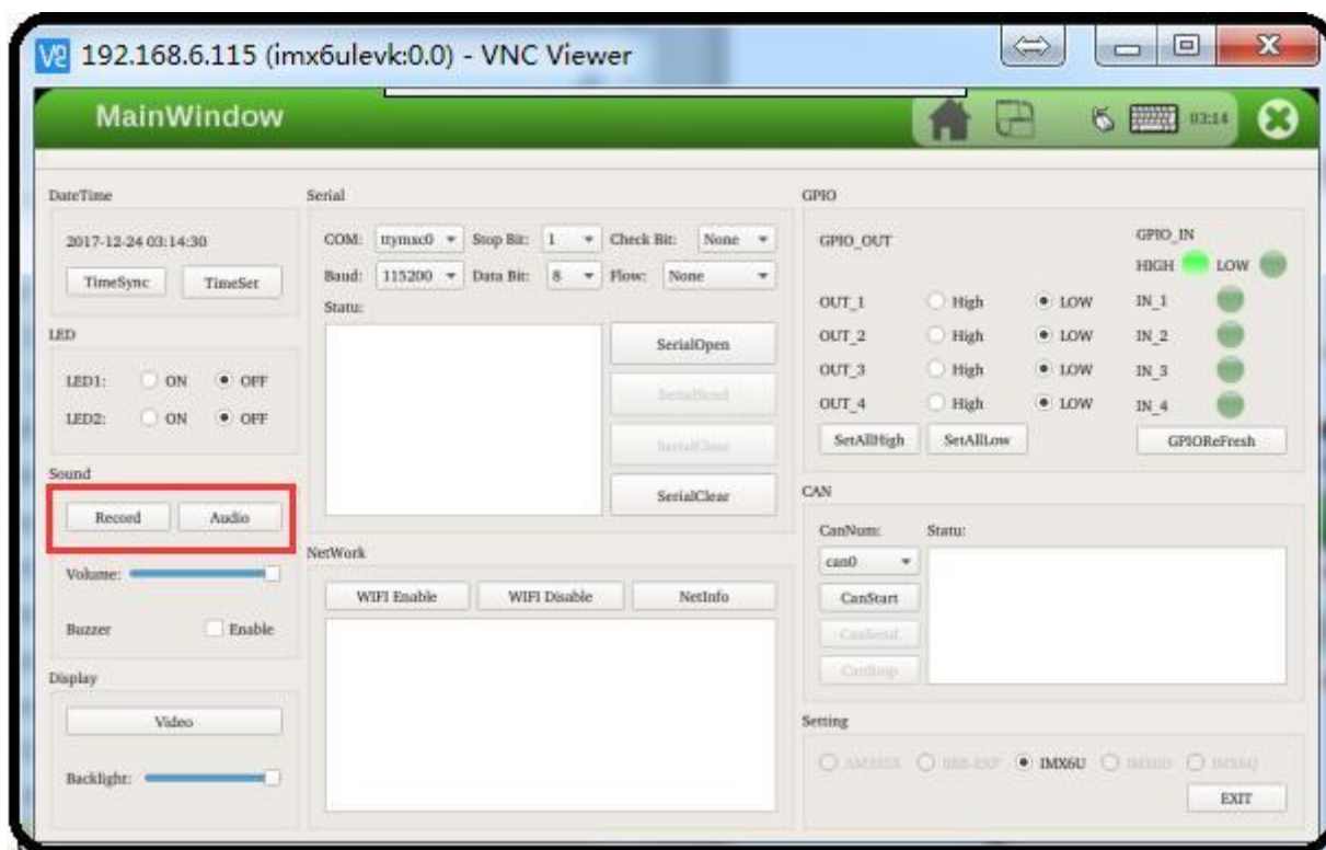
Figure 371: Audio Test
