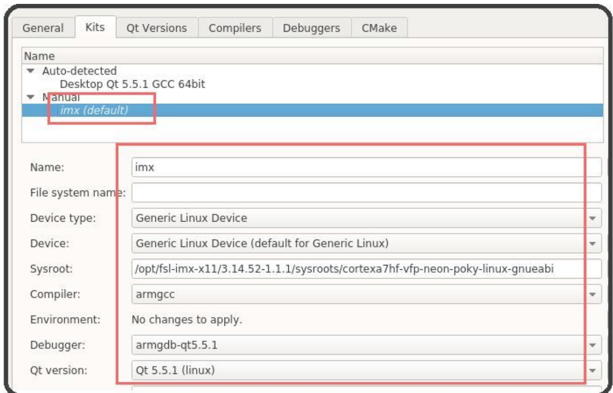
Figure 382: Kits
