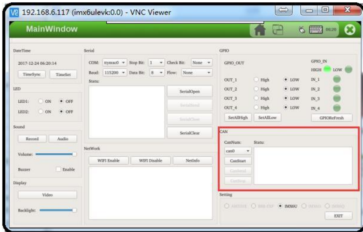
Figure 375: CAN
