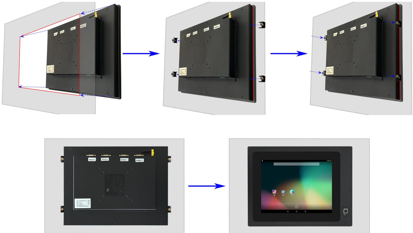
Figure 77: Panel mounting
