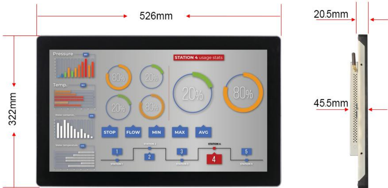
Figure 586: PPC-A72-215-C Technical Drawing
