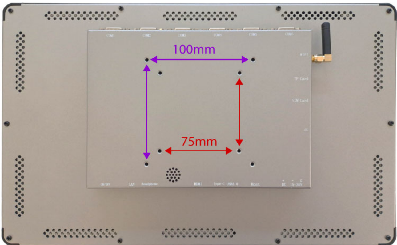
Figure 572: Mounting Method
