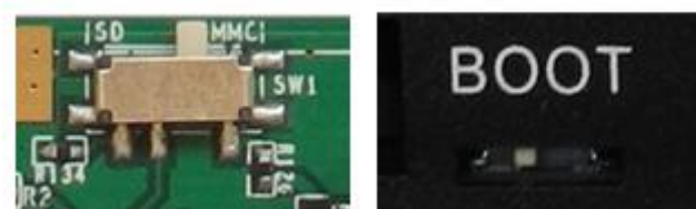
Figure 749: Boot DIP Switch
