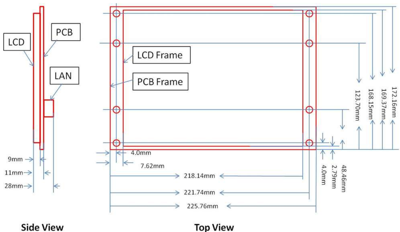
Figure 750: EPC-A8-097-C Technical Drawing
