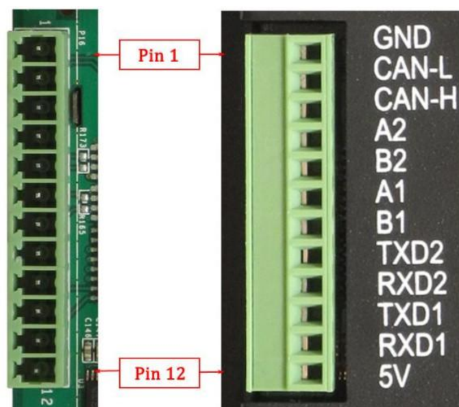
Figure 699: Relation between serial pins on embedded vs. enclosed version of the EPC/PPC-A8-070H-C Industrial PC
