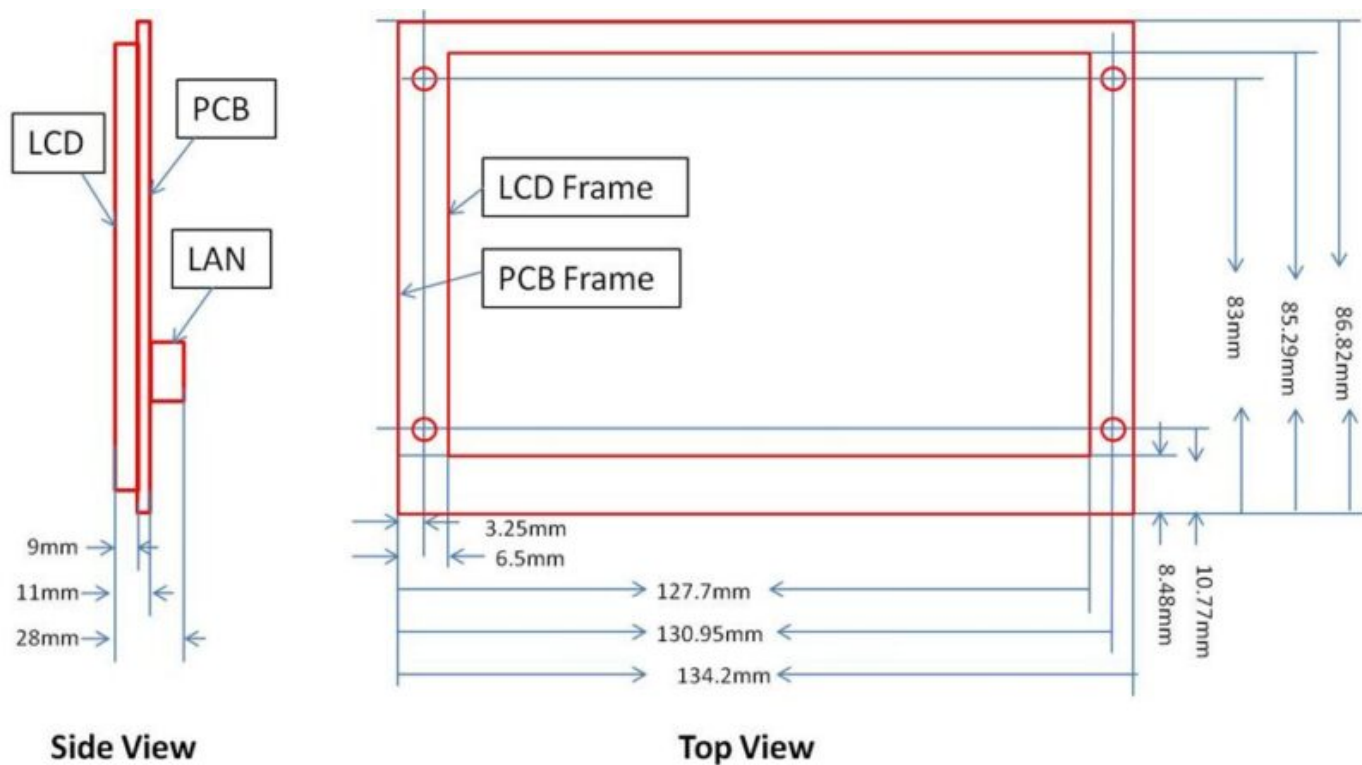
Figure 665: EPC-A8-050-C Technical Drawing
